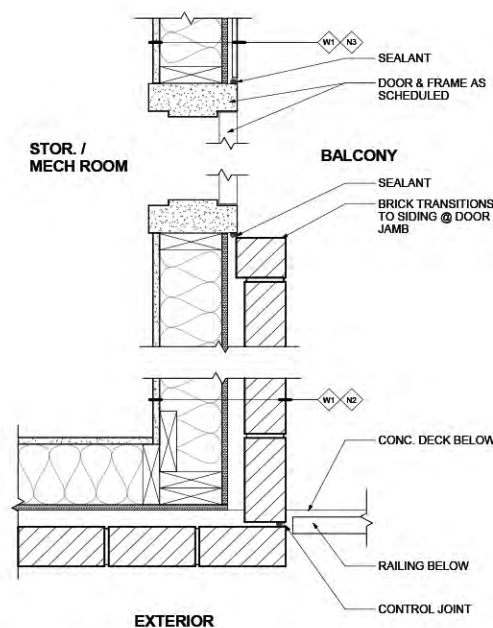
3 TYPICAL BRICK CORNER @ BALCONY 1 1/2" = 1'-0"
