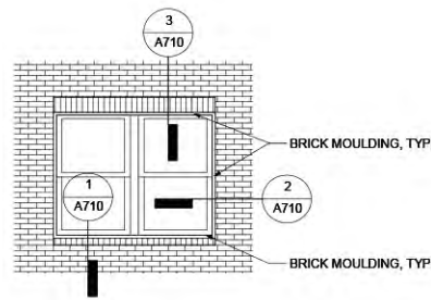
TYPICAL WINDOW ELEVATION DETAIL @ BRICK 1/4" = 1'-0"
